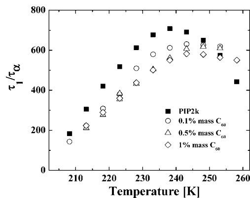
Figure 4. Ratio of chain to segmental relaxation times as a function of temperature for PIP2k with different C 60 concentrations: filled square, neat PIP2k; circle, 0.1% mass C 60 ; triangle, 0.5% mass C 60 ; diamond, 1% mass C 60 .
